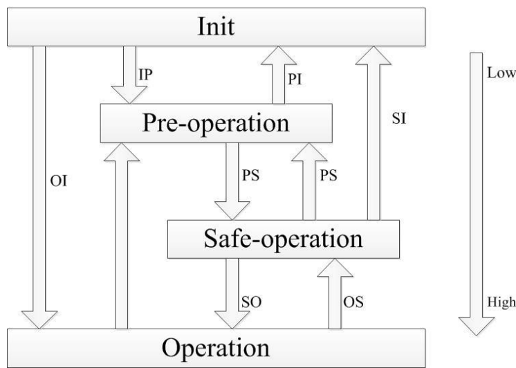
EtherCAT state machine transmission flow chart
